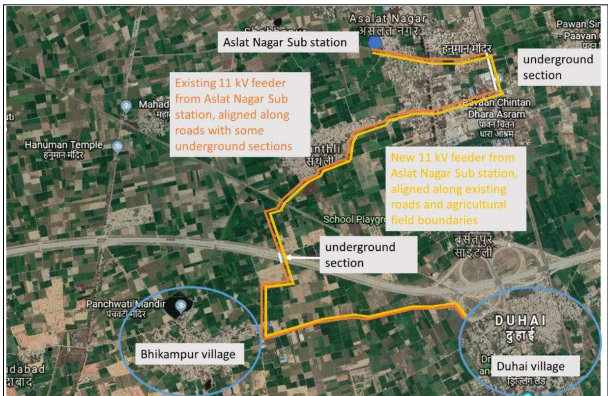
Map 7: Duhai Feeder from Aslat Nagar Sub station in DVVNL
