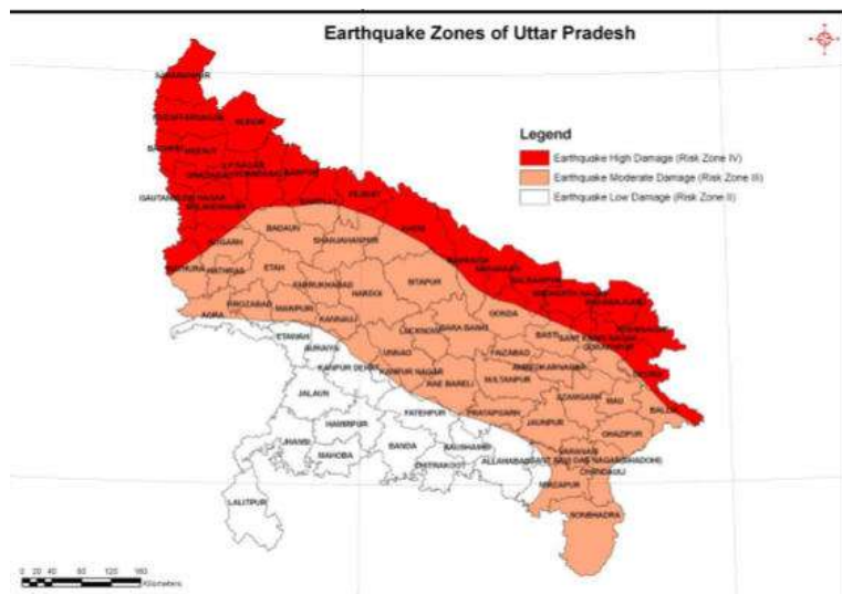
Figure 5: Seismic Zone Maps of Uttar Pradesh
