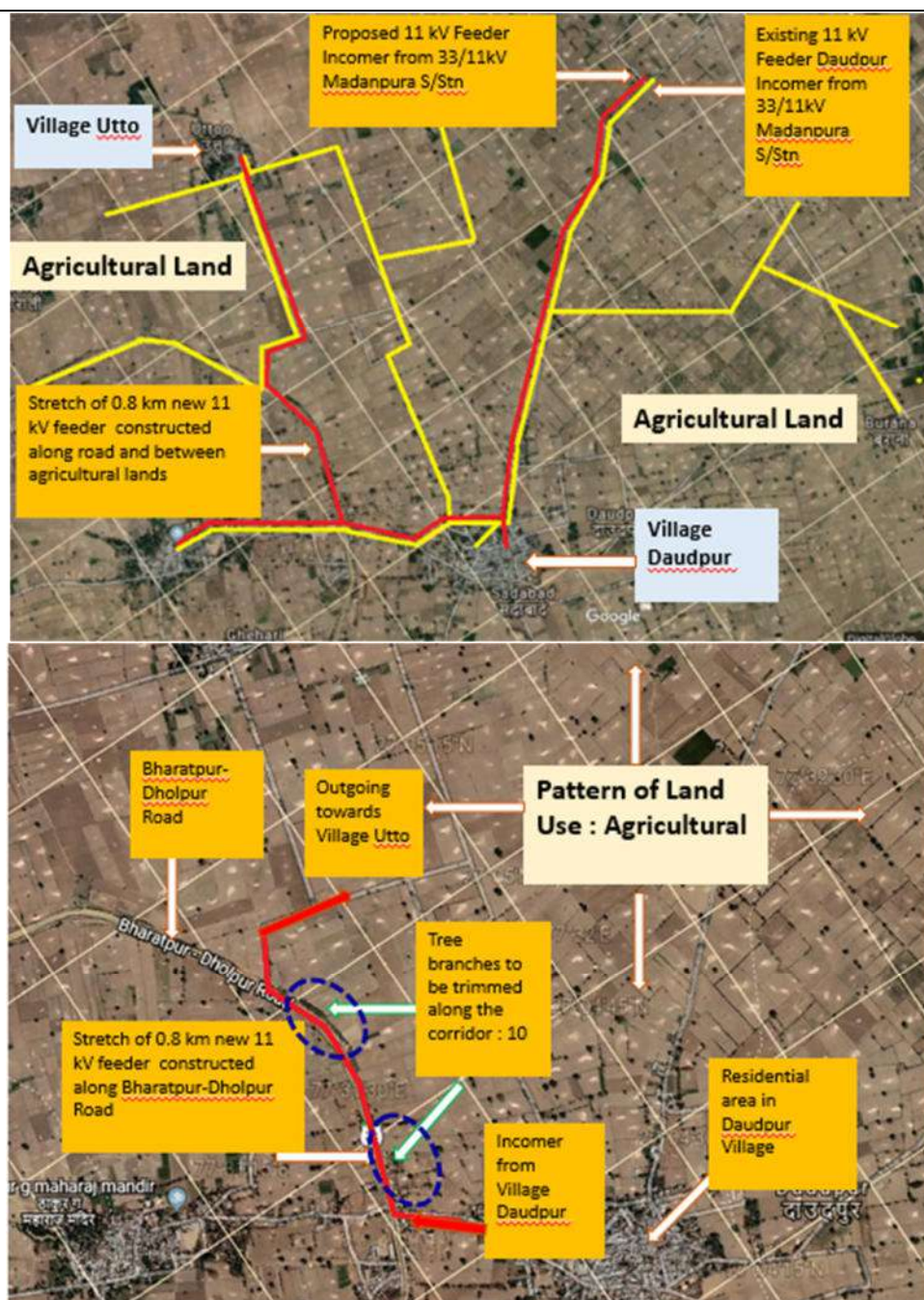
Map 1: Daudpur Feeder from 33/11 kV Madanpura substation in PVVNL
