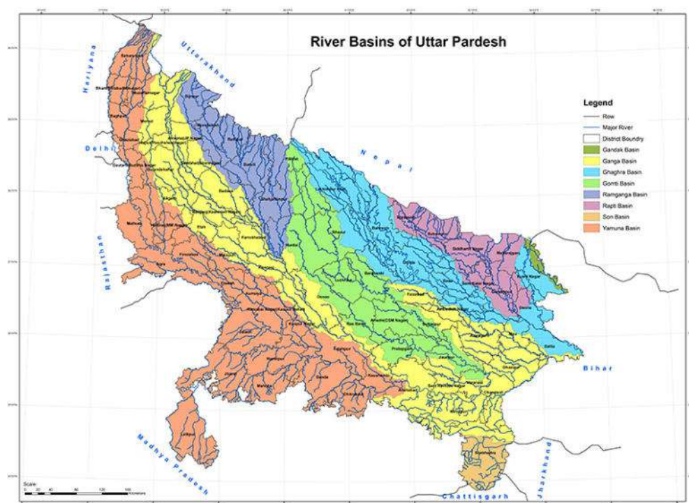
Figure 9: Drainage Map
