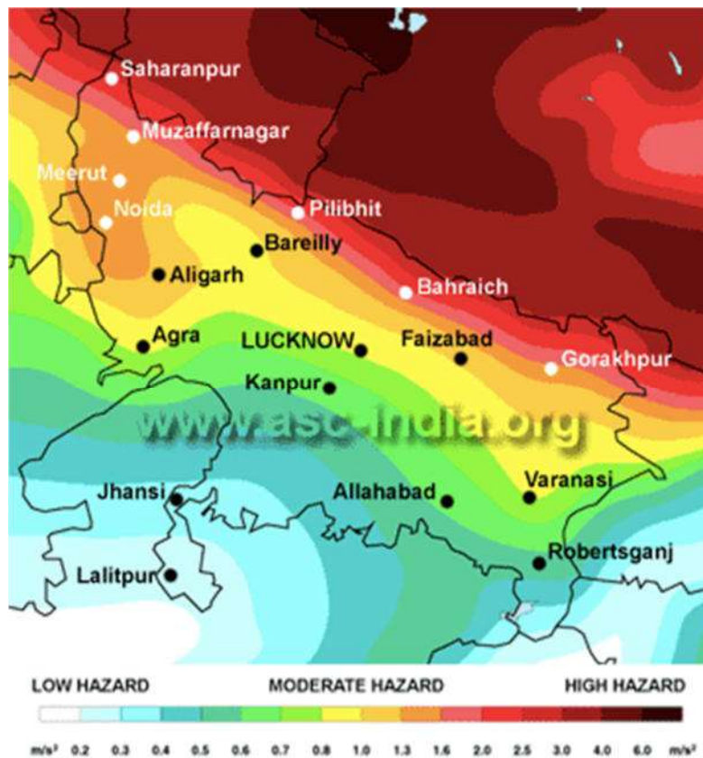
Figure 4: Hazard Risk Map of Uttar Pradesh
