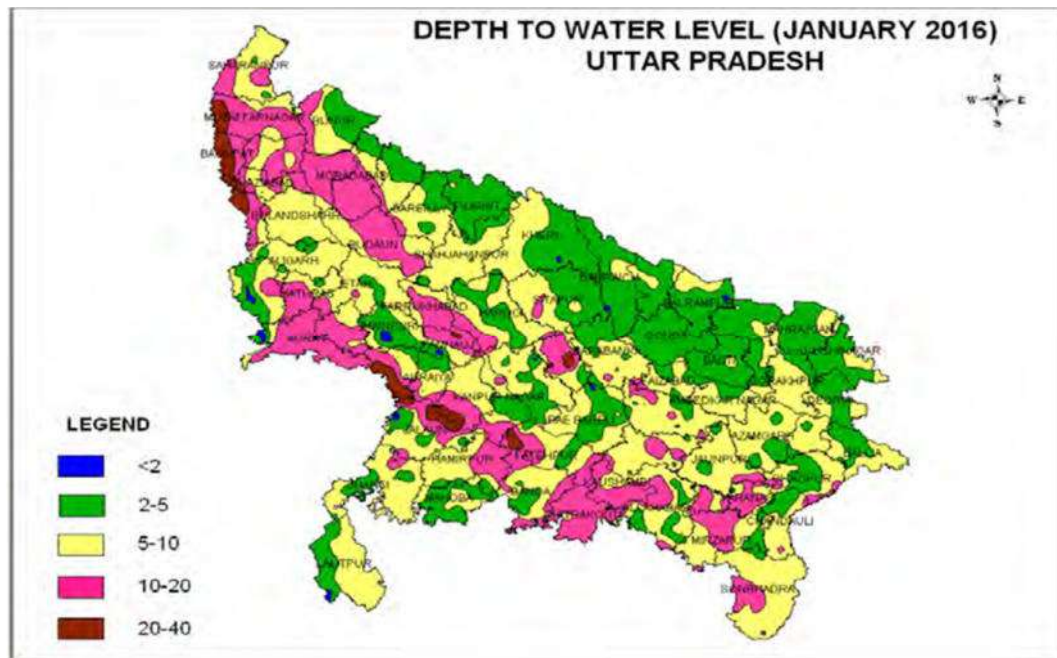
Figure 10: Groundwater Status in Uttar Pradesh
