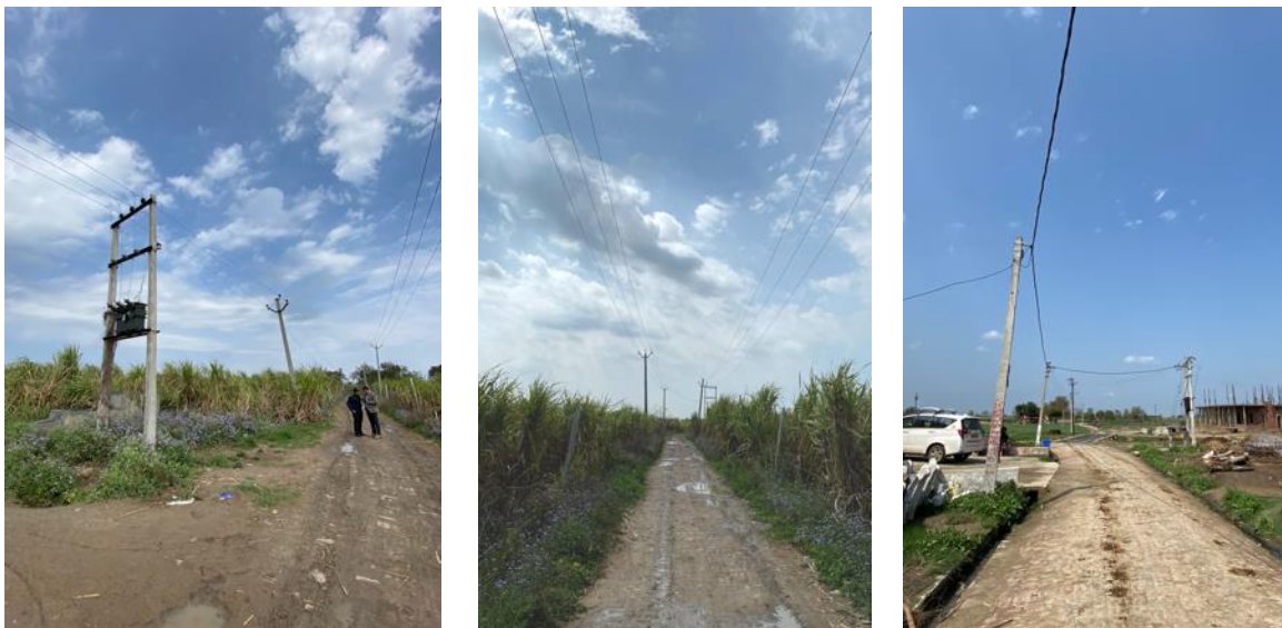
Photo 3: Completed Feeder Separation (left and middle) and ABC (right) Works
